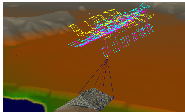
Figure 6: Spectrometer measurements from Ny-Ålesund on Svalbard.
