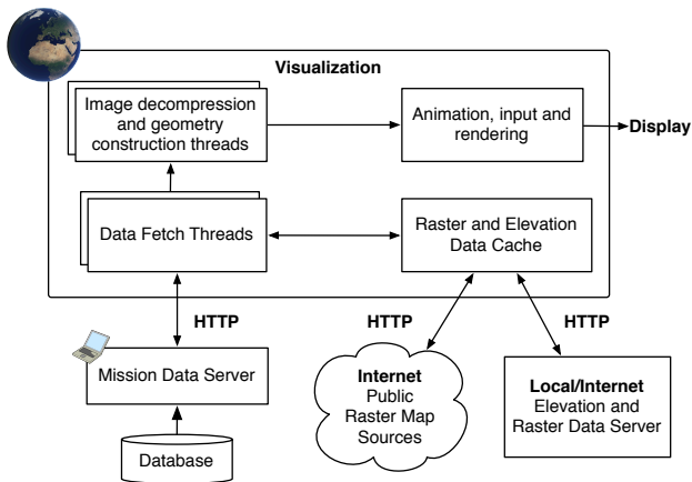
Figure 4: The visualization's design.
