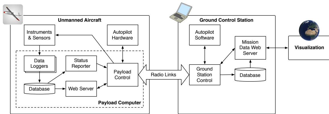
Figure 2: The overall system architecture of Norut's unmanned systems.
