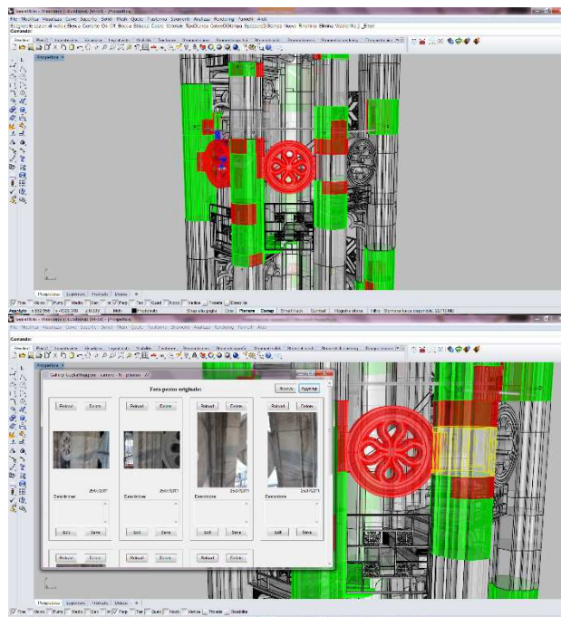
Figure 3. First part implemented inside Rhinoceros Nurbs Modeller. It is possible to see 3D models with different colour in function of different restoration activities. Info and images can be loaded and visualized with ad hoc panel. 3D model and info are loaded from the external DB and can be used without saving them locally
