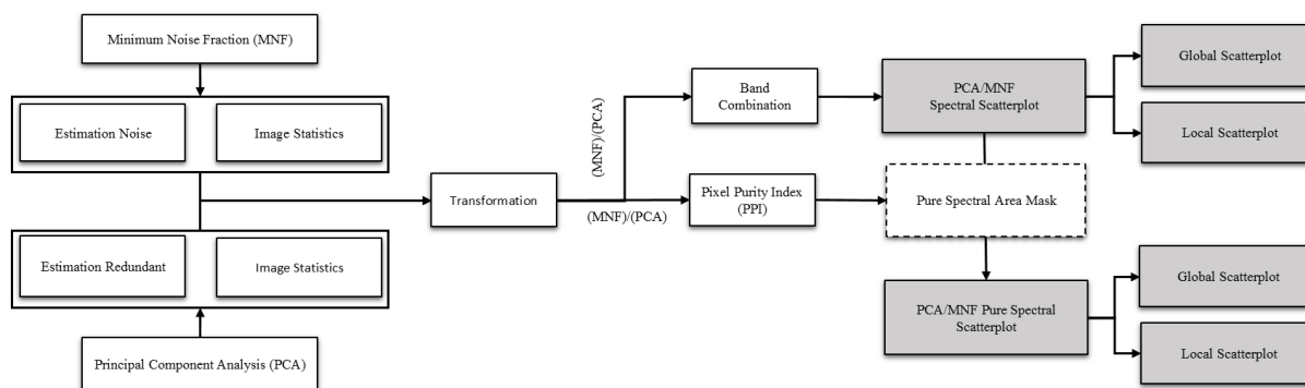
Figure 2. The process of candidate endmember selection of each endmember combination based on four strategy models: PCA/MNF Spectral + Global scatterplot, PCA/MNF spectral + Local Scatterplot, PCA/MNF pure spectral + Global scatterplot, and PCA/MNF pure spectral + Local Scatterplot.
