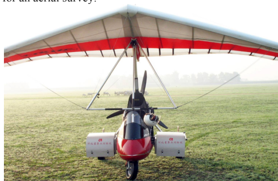
Figure 2. Microlight-Trike as a platform for aerial surveying for monitoring earthquake disasters in China
