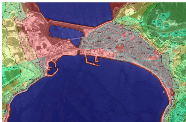
Figure 3. Tsunami Run-up simulation an area near Istanbul (Kemper et al., 2005) calculated by Land-use data (Kasanko et al., 2000) and DTM by basic equations (Heitner, 1969)
