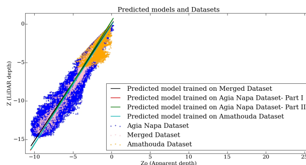
Figure 6. The Z-Z_o distribution of the employed datasets and the respective predicted linear models
