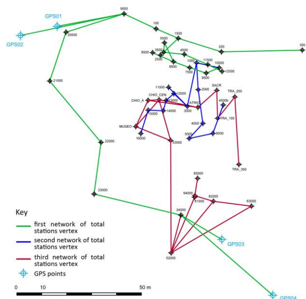
Figure 2. Network connections between total stations vertex and GNSS points
