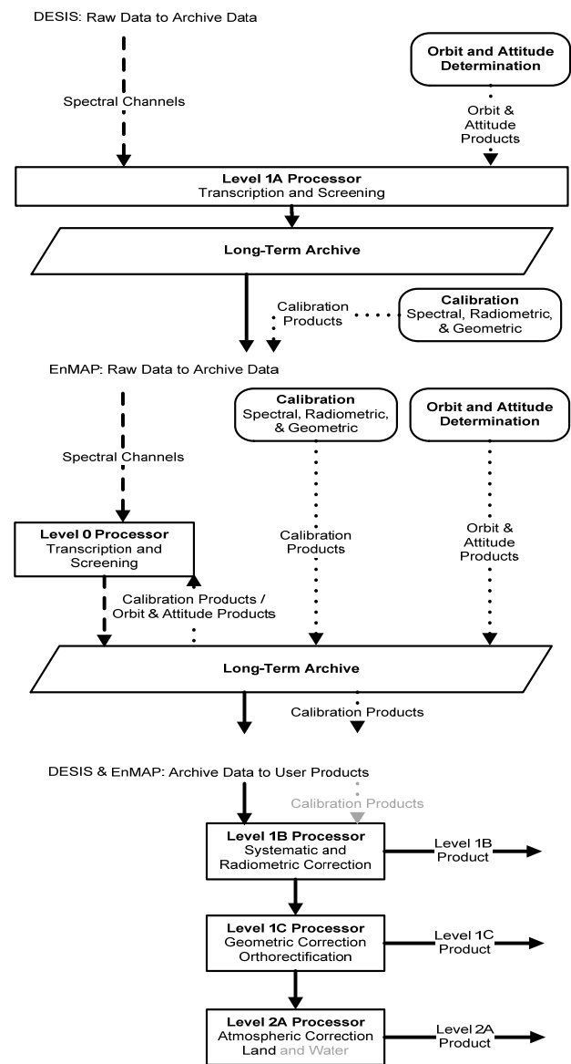
Figure 2. Image Processing Chains
