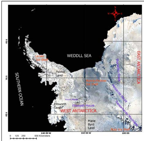
Figure 2. RGB colour combination of bands 3, 5 and 7 derived from orthorectified Landsat 7 mosaic image of West Antarctica.
