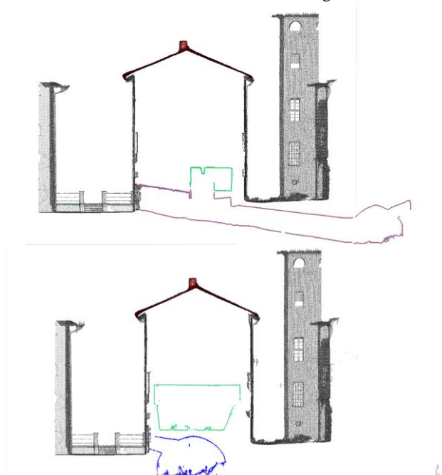
Figure 14. Section profile on UAV, LiDAR and ZebRevo clouds.
