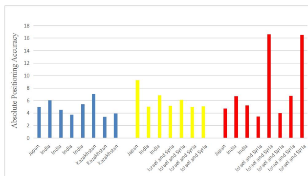
Figure 3. Absolute positioning accuracy distribution on plains (blue columns), hills (yellow columns), and mountain (red columns) terrain
