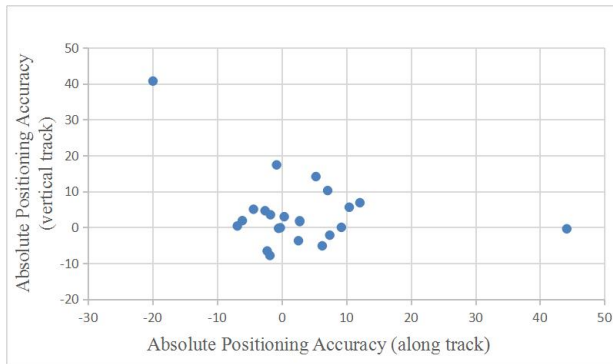
Figure 5. Spatial distribution of absolute positioning accuracy in GE's imagery
