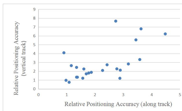
Figure 4. Spatial distribution of relative positioning accuracy in GE's imagery
