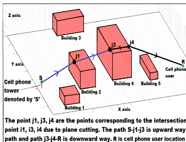
Figure 6. A signal path over the top of buildings
