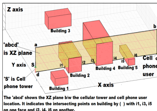
Figure 5. XZ plane intersecting with Building present
