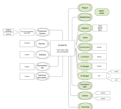
Figure3 Scheme of WH list data model.
