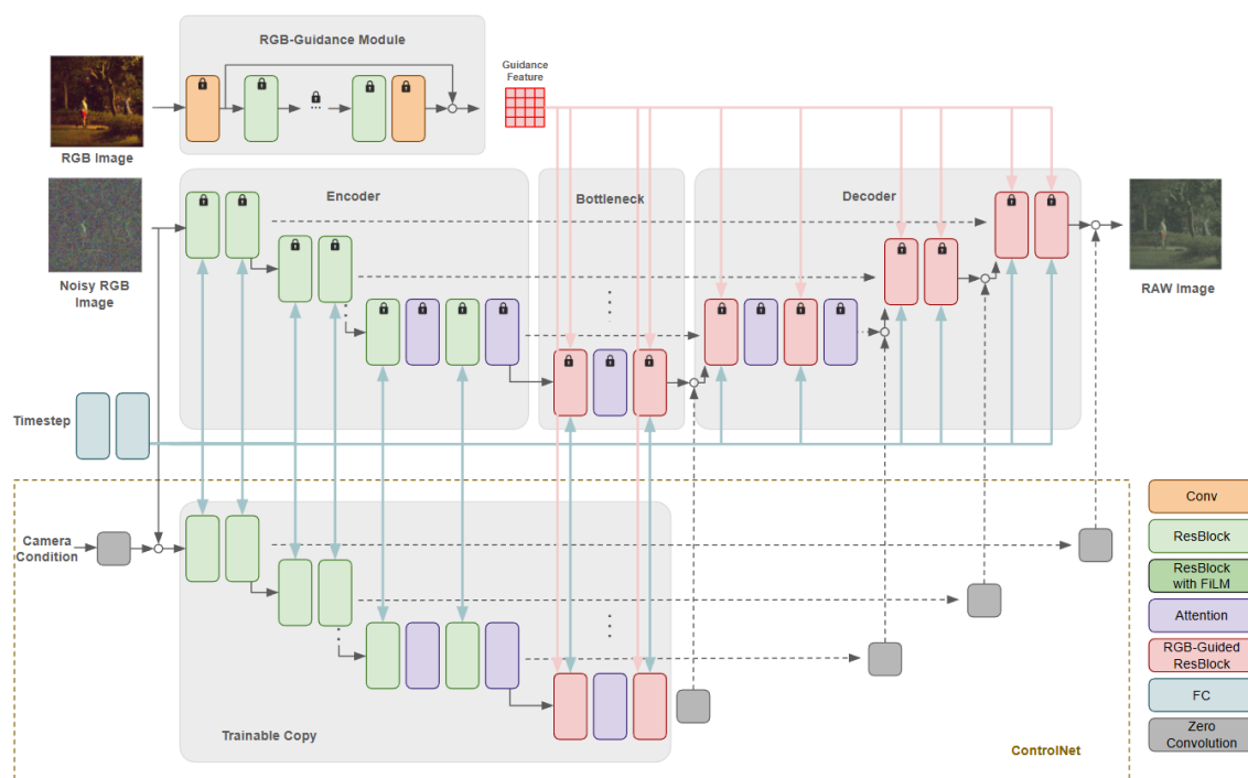
Figure 3. Raw-Diffusion with ControlNet Injection. The upper pathway is the frozen RGB-guided RAW-Diffusion backbone; the lower pathway is the trainable ControlNet, which produces multi-scale residuals that are passed through zero convolutions.
