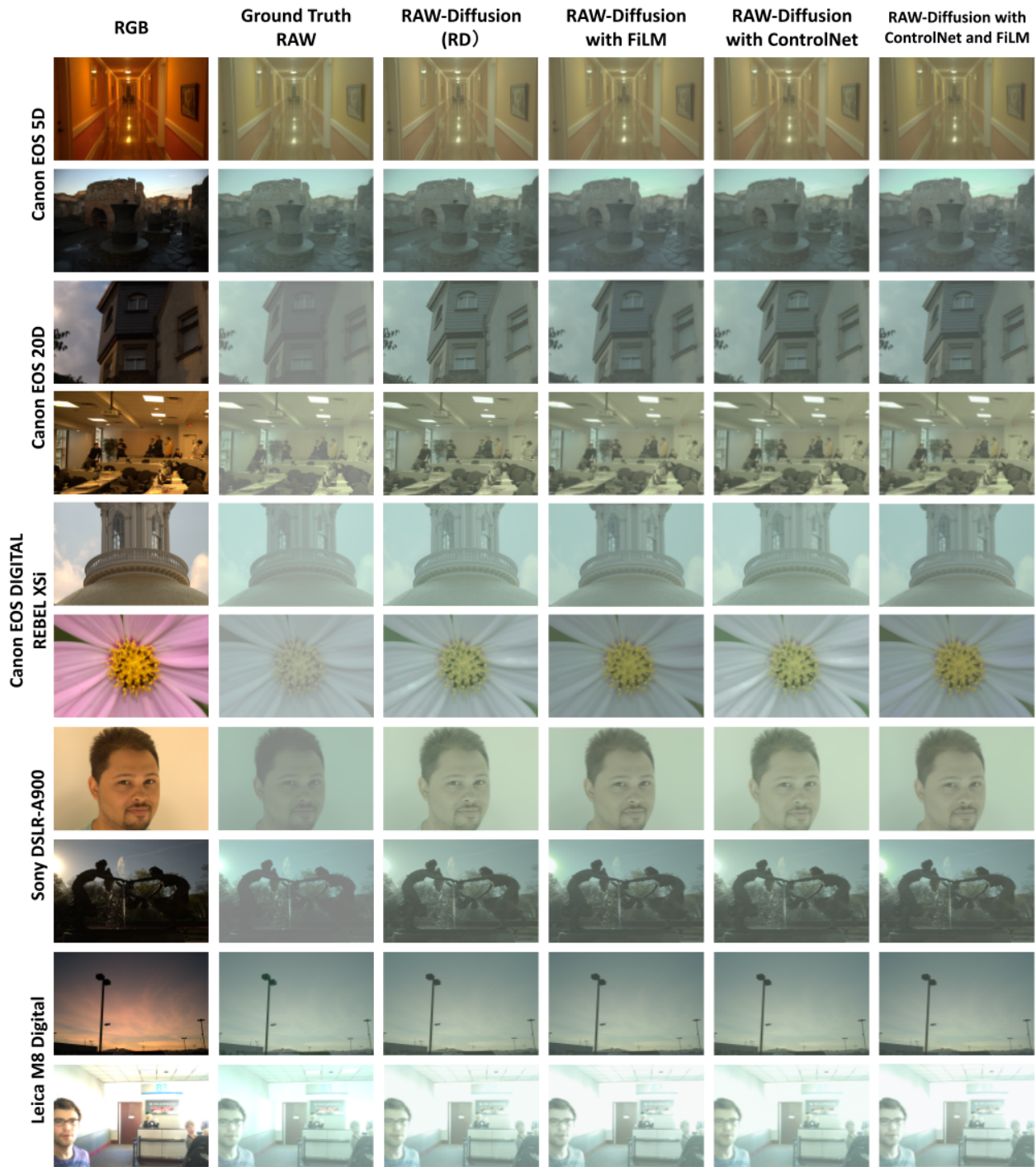
Figure 7. Qualitative comparison of RAW reconstruction across different model variants.
