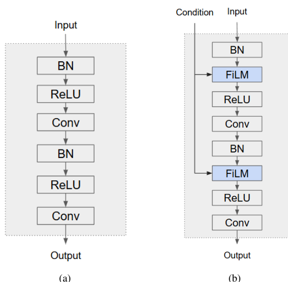
Figure 4. (a) Original Residual Block; (b) Residual Block with Feature-wise Linear Modulation (FiLM).
