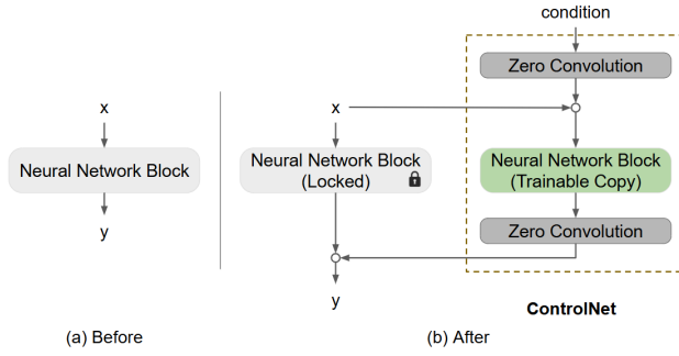
Figure 2. ControlNet: (a) A neural network block maps an input feature map x to an output feature map y . (b) The parameters of the original neural network block are frozen. We create a trainable copy and link x and y using zero-convolution layers, i.e., 1 \times 1 convolutions whose weights and biases are initialized to zero.
