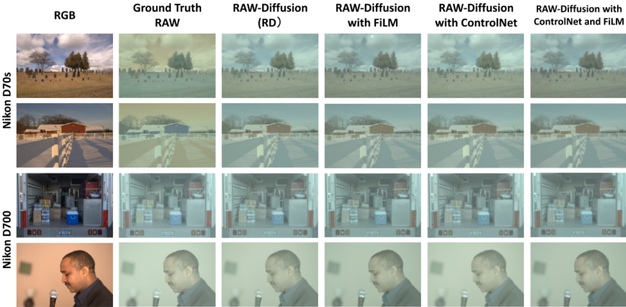
Figure 6. Qualitative comparison of RAW reconstruction across different model variants.
