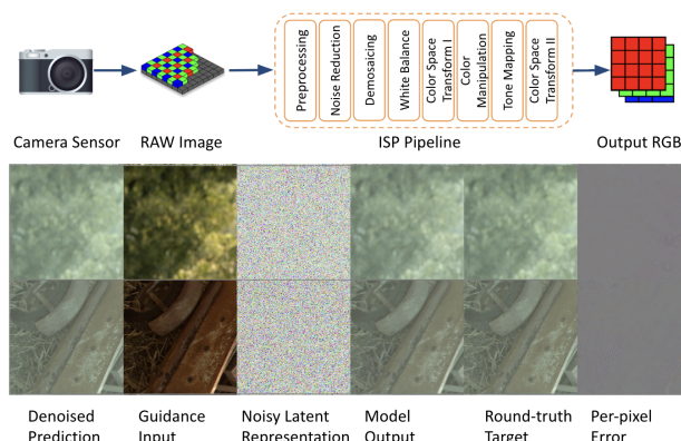
Figure 1. The top row illustrates a typical camera ISP pipeline. The bottom row shows an example visualization during training.
