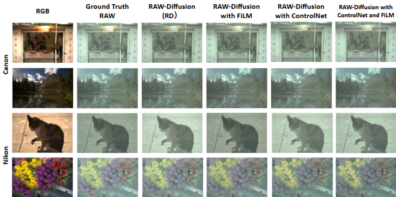
Figure 5. Qualitative comparison of RAW reconstruction across different model variants. From left to right: input sRGB image, ground-truth RAW, RAW-Diffusion (RD), RAW-Diffusion with FiLM, RAW-Diffusion with ControlNet (ours), and RAW-Diffusion with both ControlNet and FiLM.
