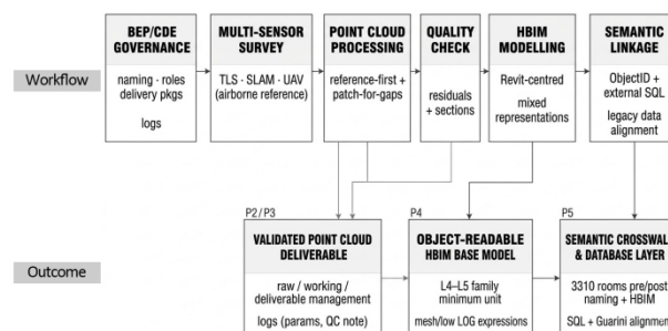
Figure 3. Proposed Scan-to-BIM Workflow overview
