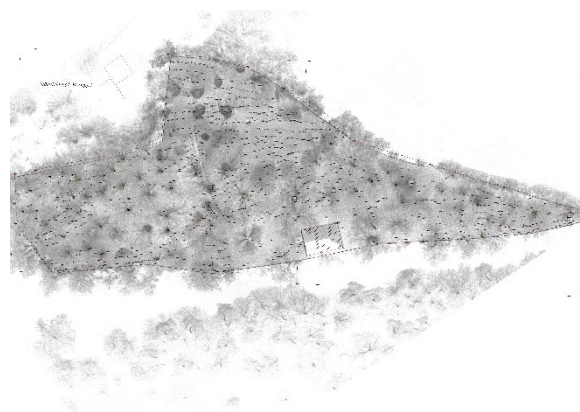
Figure 4. Extraction of a plan from 3D mobile laser scanning from the topographic terrain model with gravestones for an accurate representation of topography and spatial arrangement of gravestones, Jewish Cemetery Walsdorf.
