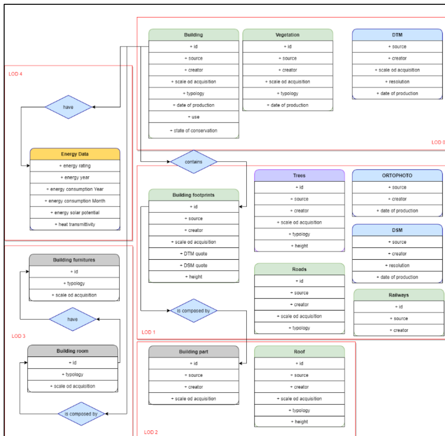
Figure 5. Conceptual model for the GeoDB creation.
