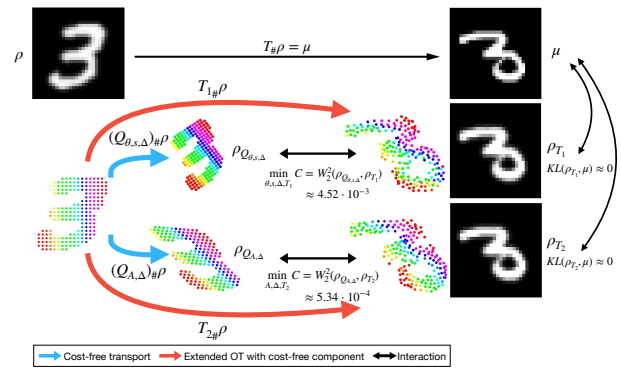
Figure 5. Two gray-scaled, hand-written digits 3 in different styles as the source and the target. The middle column displays cost-free components from the family of linear combinations of rotation, scaling, and translation, and the corresponding completion of the map. The right column shows the cost-free affine transformation and the corresponding unrestricted push forward map.
