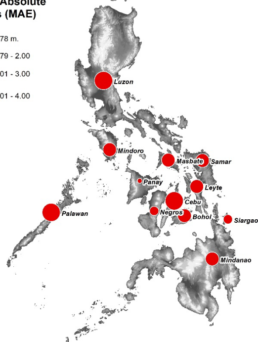
Figure 7. FABDEM MAEs at selected islands of the Philippines. The values illustrated are the average of the MAE calculated from the three sets of GCPs.
