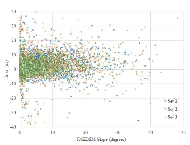
Figure 5. FABDEM errors plotted versus slope.
