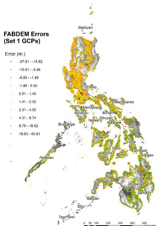
Figure 2. Spatial distribution of FABDEM errors at Set 1 GCP locations.
