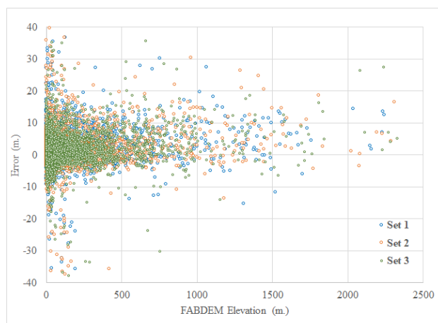
Figure 4. FABDEM errors plotted versus elevation.
