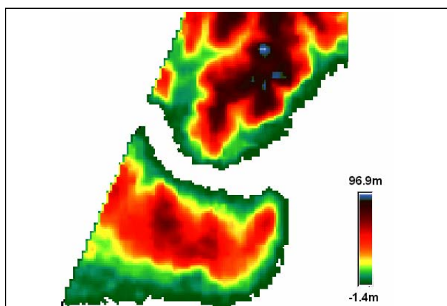
Figure 8. SRTM C-band height model of Istanbul
